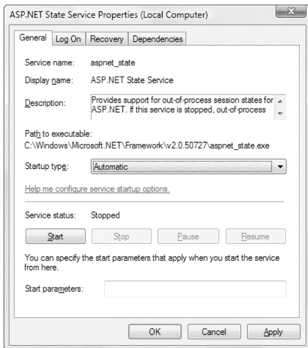
Figure 6-7. Service properties
