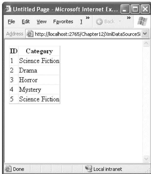
Figure 14-10. Flattening XML with data binding
