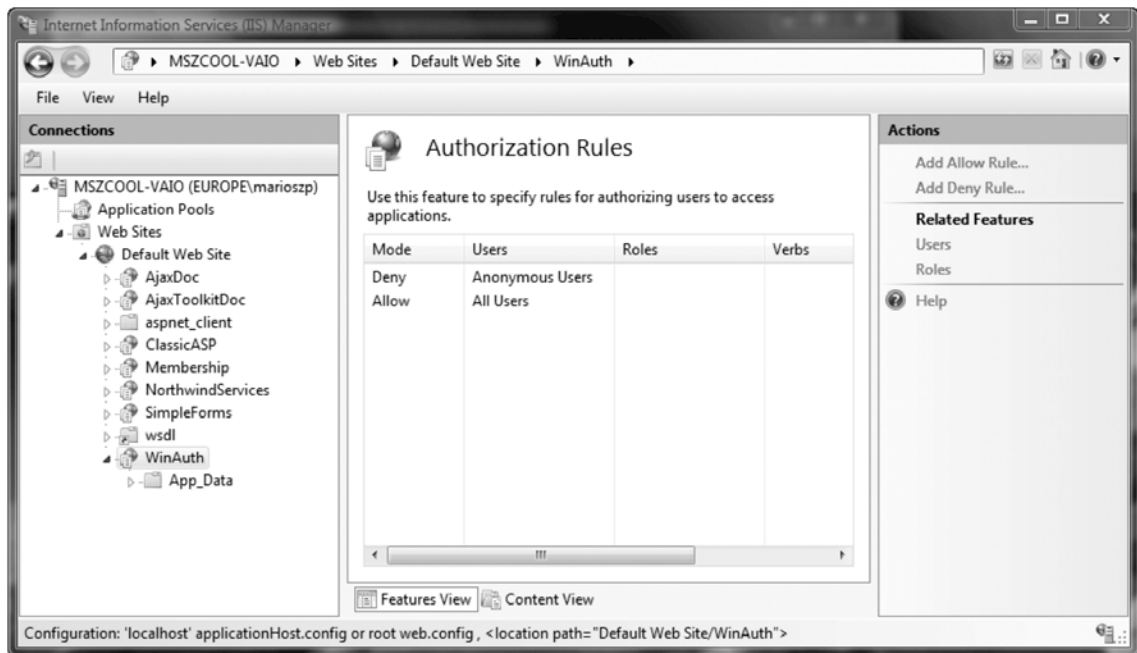
Figure 22-10. IIS authorization configuration for Windows authentication
