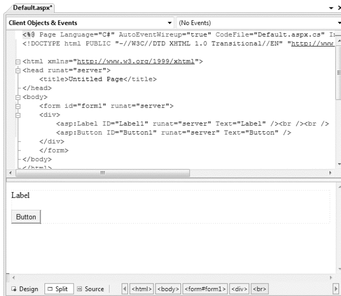
Figure 2-3. Editing a web page in split view
