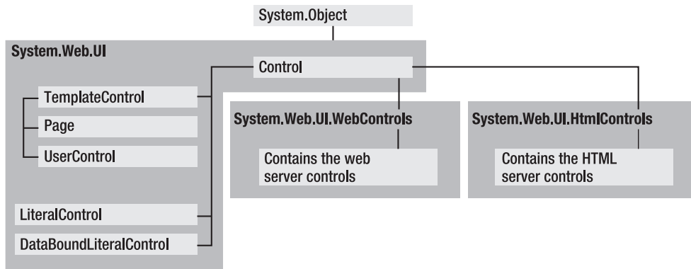
Figure 4-1. Server control inheritance
