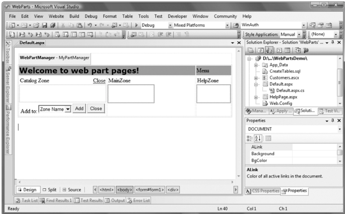
Figure 31-3. Web part pages in the Visual Studio designer
