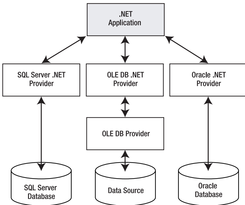
Figure 7-1. The ADO.NET architecture
