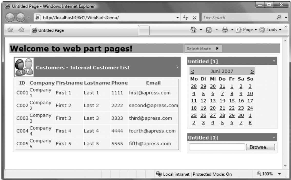
Figure 31-9. Customized Customers web part through the interface implementation
