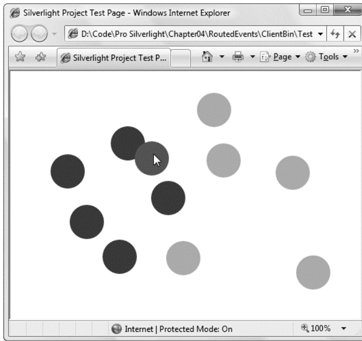
Figure 34-9. Dragging shapes
