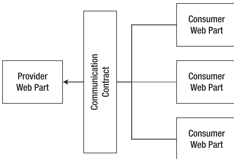
Figure 31-15. The pieces for creating connectable web parts
