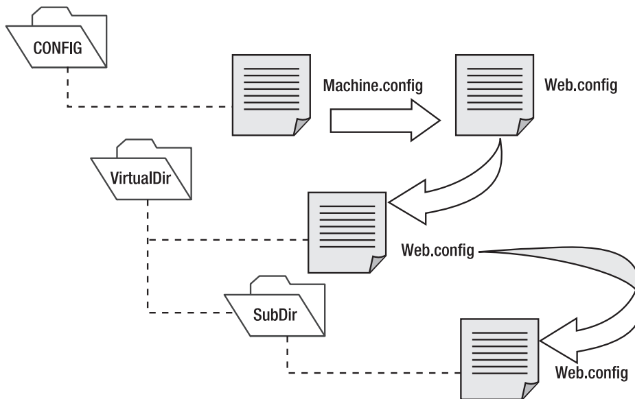
Figure 5-3. Configuration inheritance
